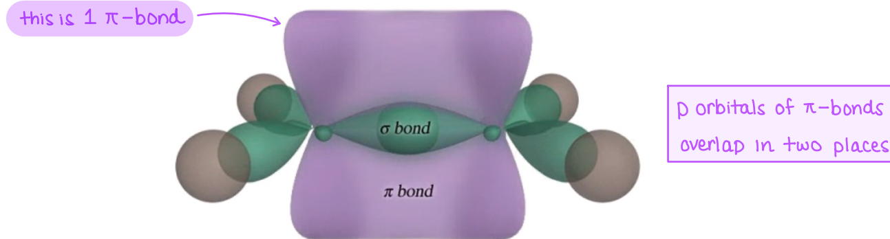
FIGURE 11.27 One \pi -bond in \text{H}_2\text{C}=\text{CH}_2
