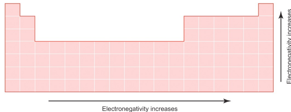
FIGURE 11.15 Electronegativity Trend
