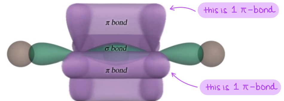
FIGURE 11.30 Two \pi -bonds in \text{HC}\equiv\text{CH}
